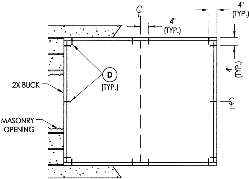
BUCK ANCHORING
