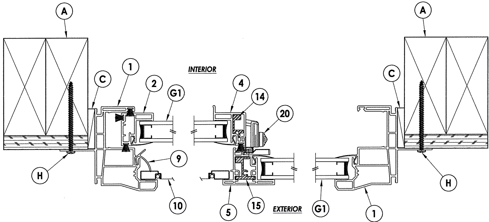
1 3 HORIZONTAL CROSS SECTION Stud Construction
