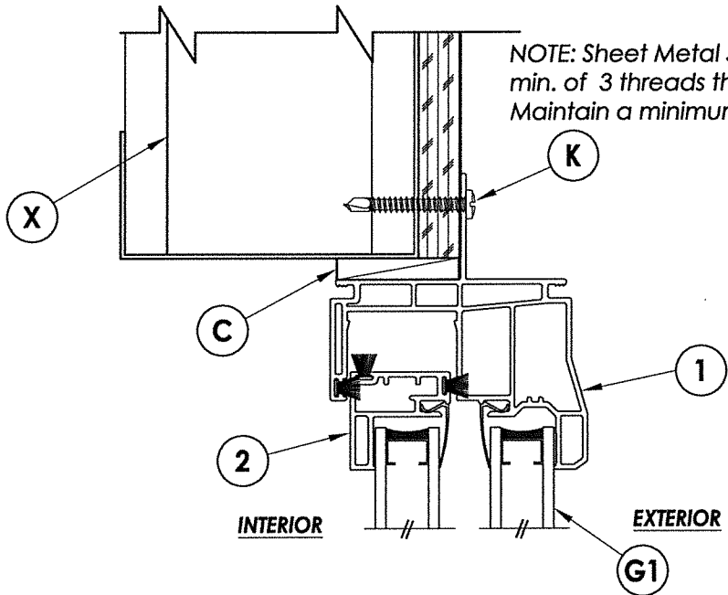
3 3 VERTICAL CROSS SECTION Steel Stud Construction
