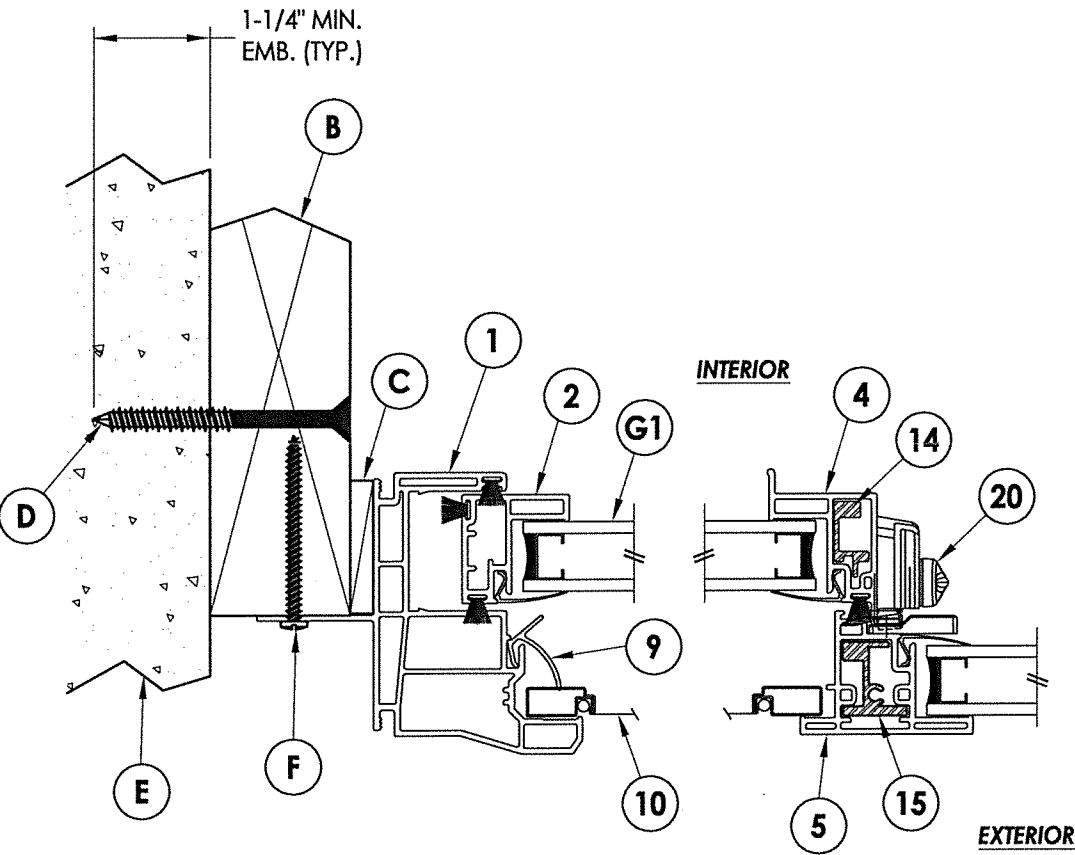
1 HORIZONTAL CROSS SECTION 2 2x Buck Construction
